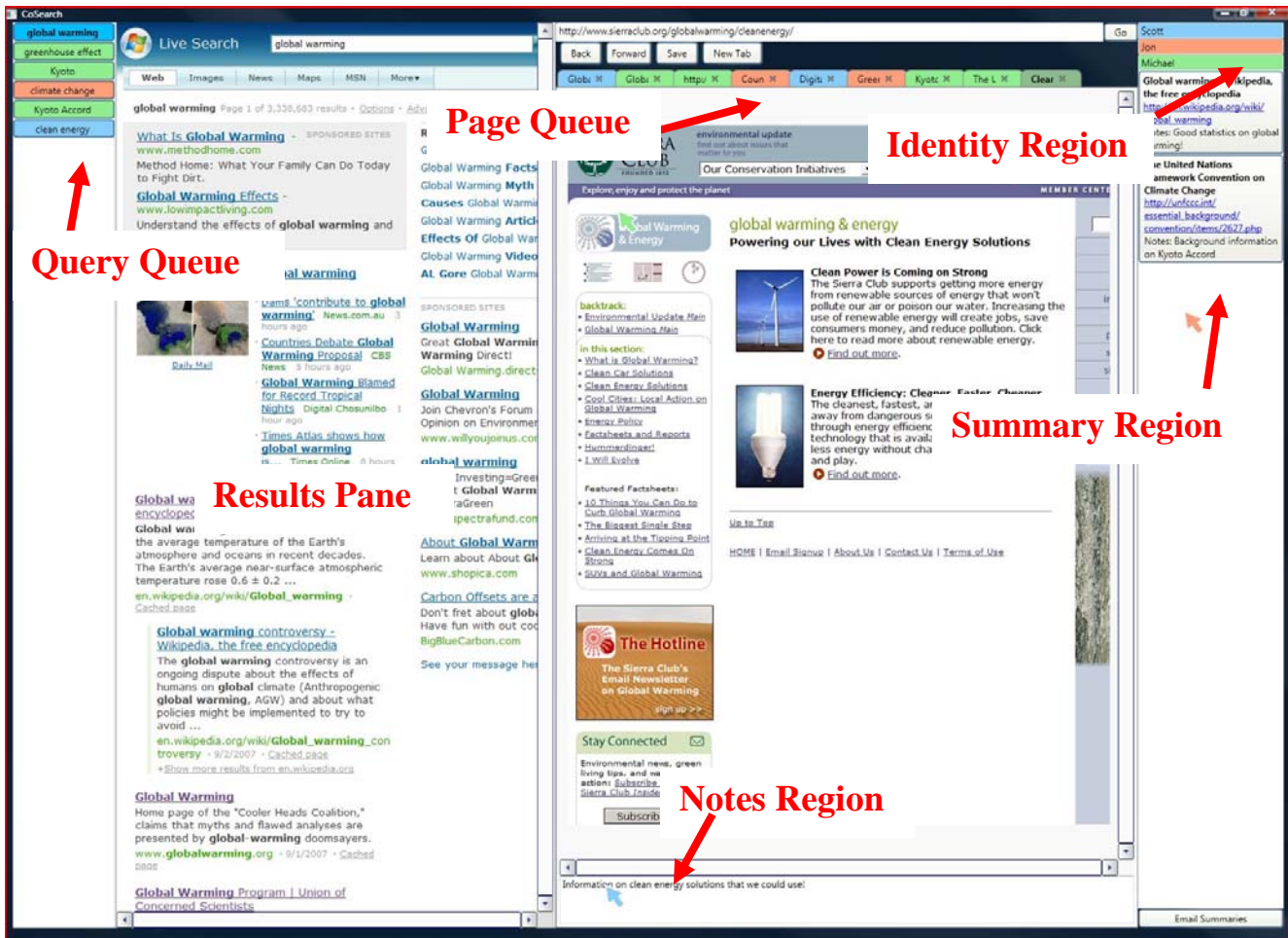
Figure 1. CoSearchPC, with annotations identifying key UI features.
